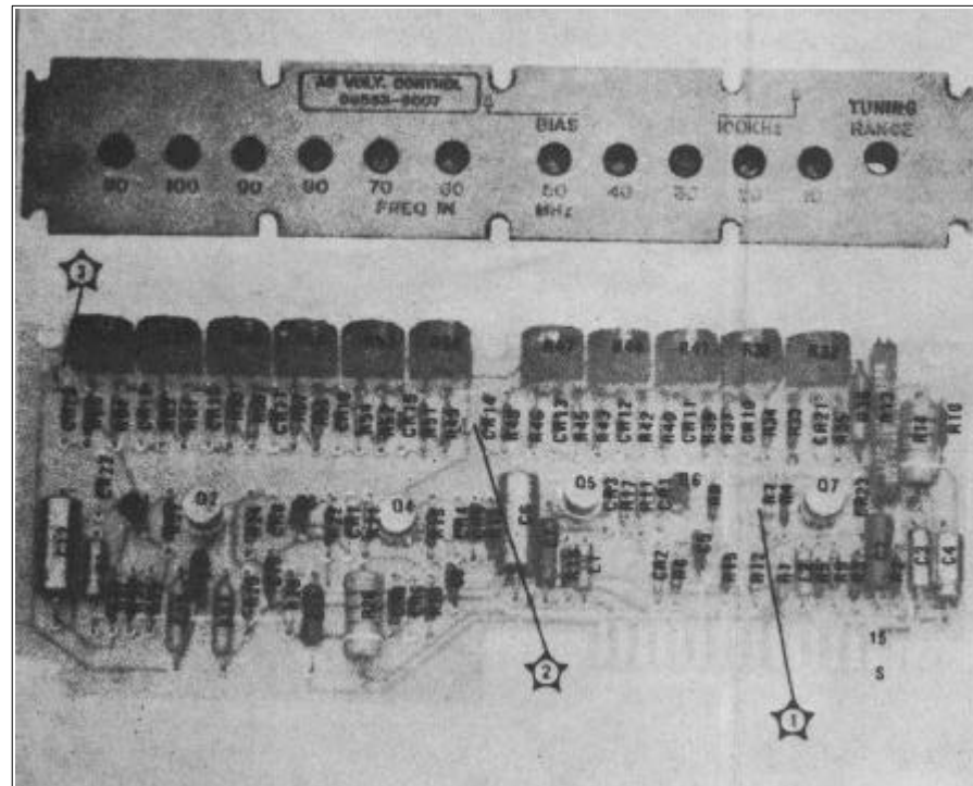
Figure 8-41. Voltage Control A5 (08553-6007) Adjustments, Test Points and Component Locations.
