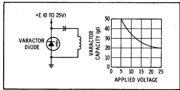
Figure 8-12. Varactor Characteristics.
