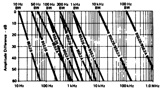
Figure 1-3. Typical Resolution
