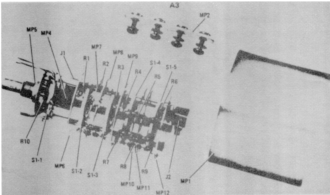
Figure 8-24. Input Attenuator Assembly A3 (08553-6021) Replaceable Parts Locations (ERRATA)
