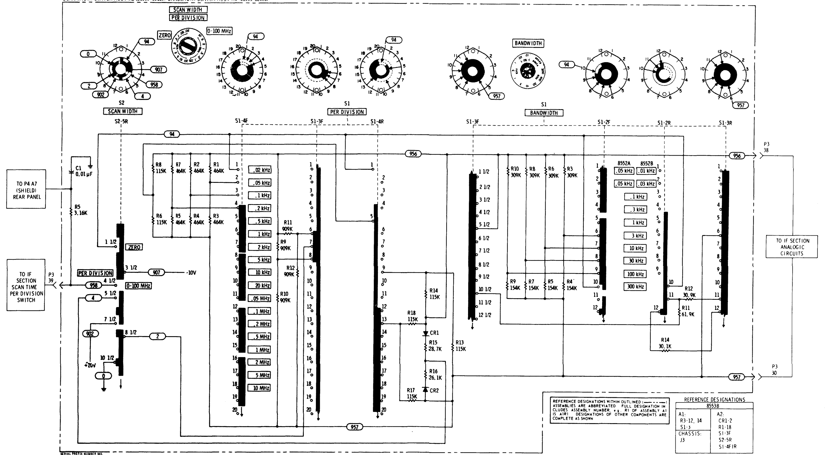
Figure 8-50. Analogic Switching Matrix
